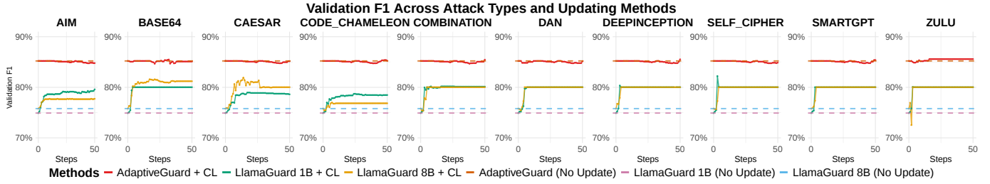
Fig. 6. (RQ3 Results) The performance comparison of our ADAPTIVEGUARD and LlamaGuard on in-distribution prompts when continuously updated through detected OOD prompts.
