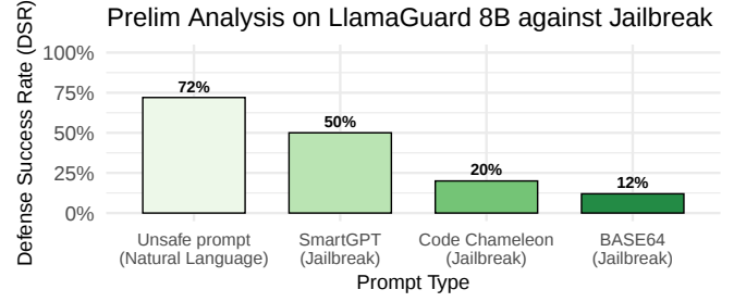
Fig. 1. DSR of jailbreak attacks on LlamaGuard-8B Guardrail.
