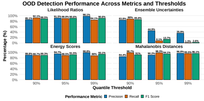
Fig. 4. (RQ1 Results) OOD detection performance of each OOD method evaluated in RQ1.
